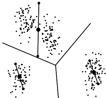
Figure 2. Each original centroid splits into two children.
